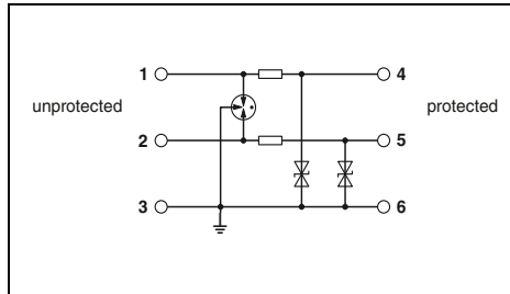
2-conductor with common reference potential, 3/6 connection grounded via gas-filled surge arrester, with or without status indicator and knife disconnection, e.g., for binary signals
