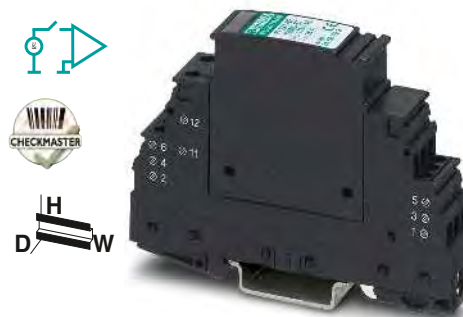
2-conductor, floating, free of leakage current, e.g., for actuator circuits
