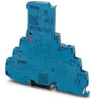
2-conductor with common reference potential, intrinsically safe, pluggable
