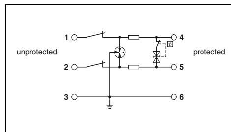
Double wire (loop), floating, 3/6 connection grounded directly, with knife disconnection, e.g., for 4 ... 20 mA current loop
