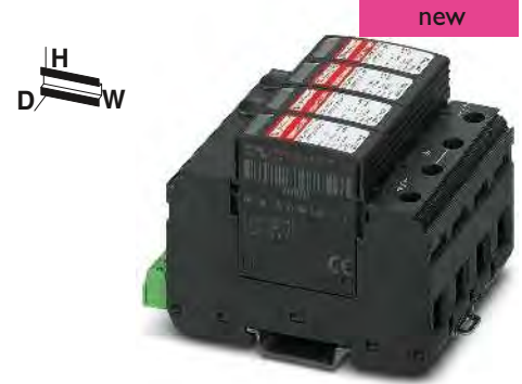
Pluggable lightning and surge protection for PV applications up to 1000 V DC
