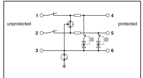
2-conductor with common reference potential, 3/6 connection grounded via gas-filled surge arrester, with knife disconnection, e.g., for binary signals
