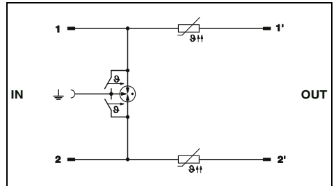
2-conductor, coarse protection, with failsafe contact and current protection (Powercross)
