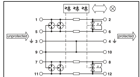
2 double wires (loops), floating, connection 9/10 grounded directly, e.g., for 4 ... 20 mA current loop
