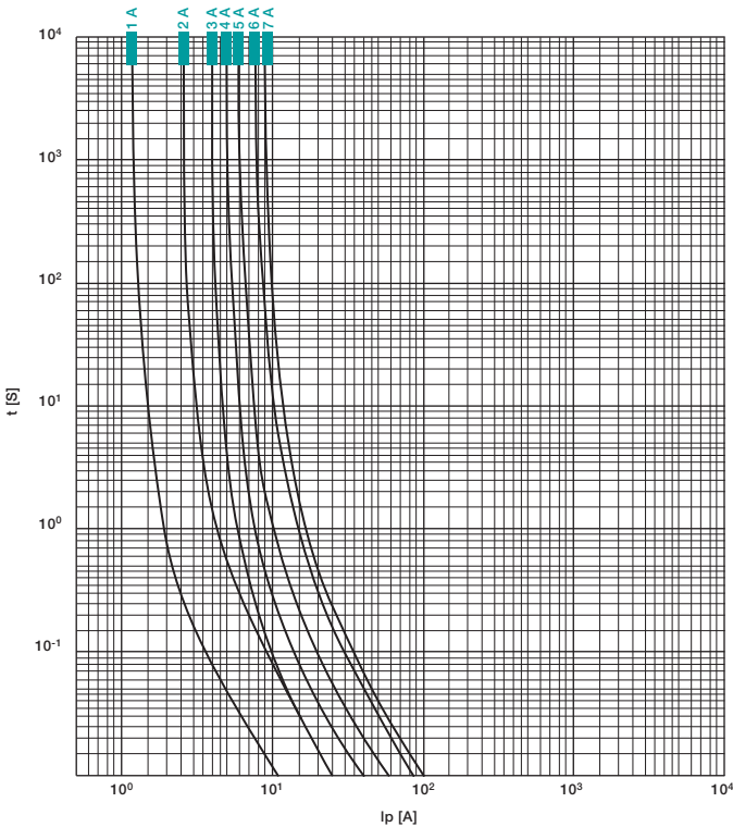
Time/current tripping characteristics
