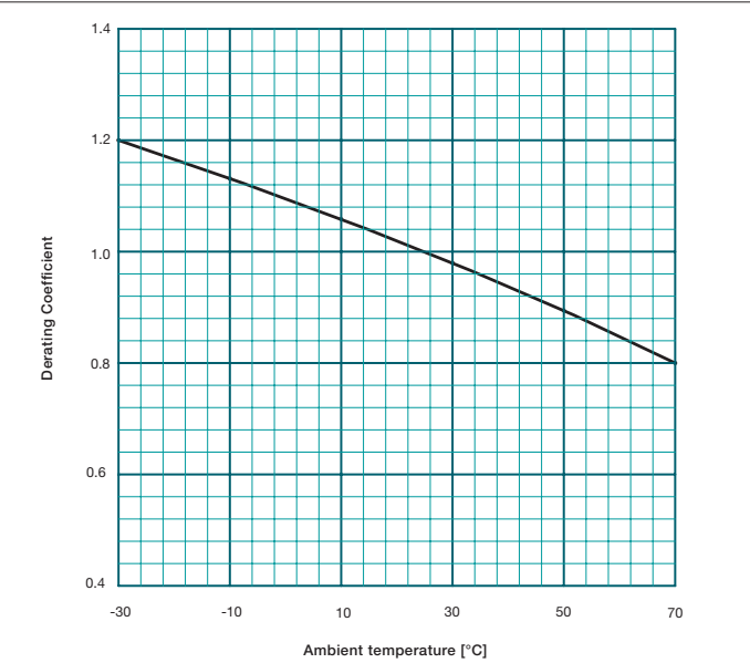
Derating in combination with ambient temperature
