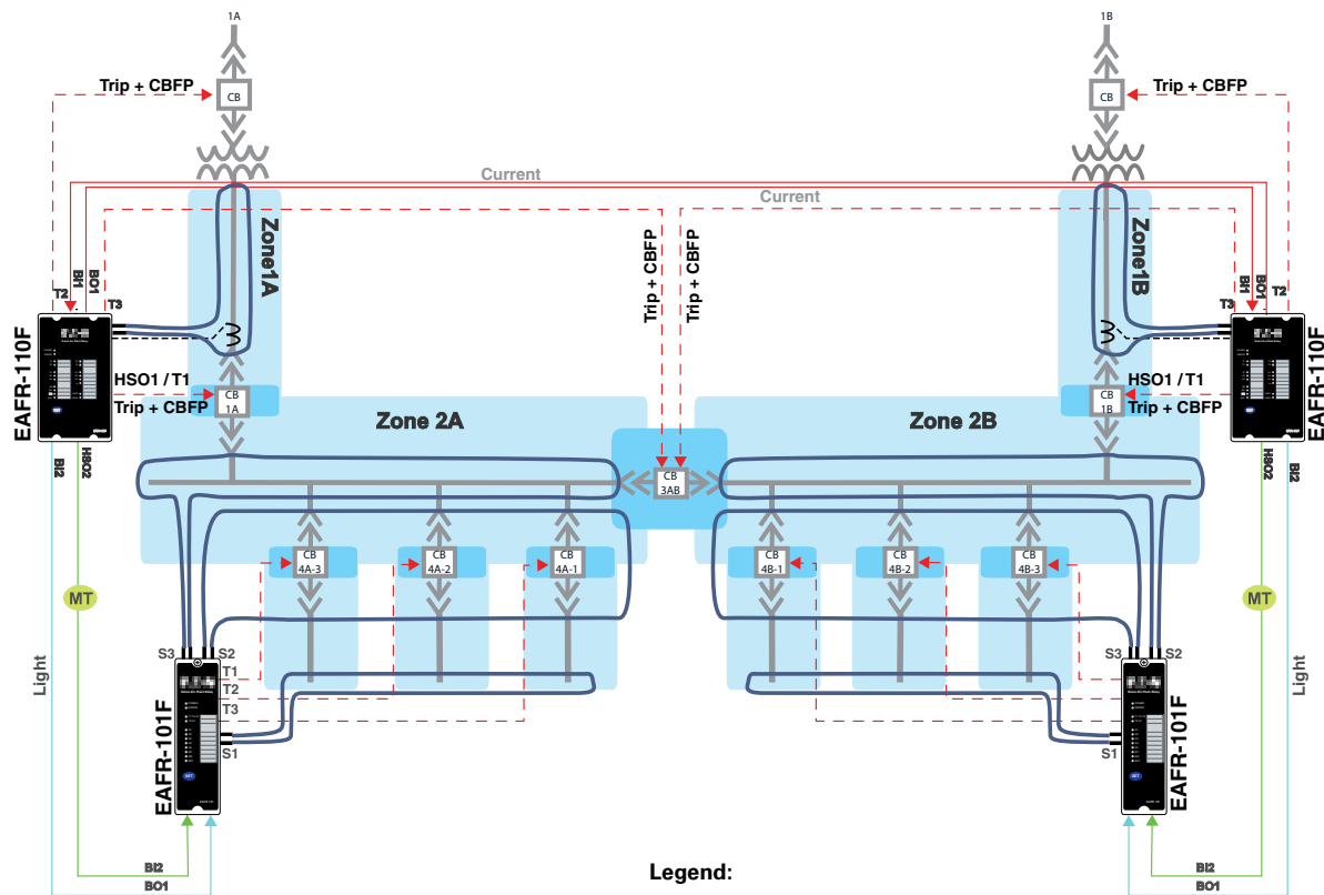
Figure 3. Double ended substation using fiber loop sensors
