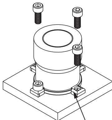
4 PAC clamps are shipped with each die set. Extra clamps can be ordered using part # PACCLAMP.
