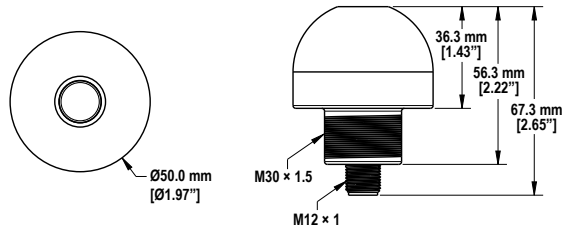
Optical Sensor
