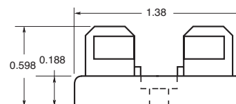
4393 spare fuse block, no terminals
