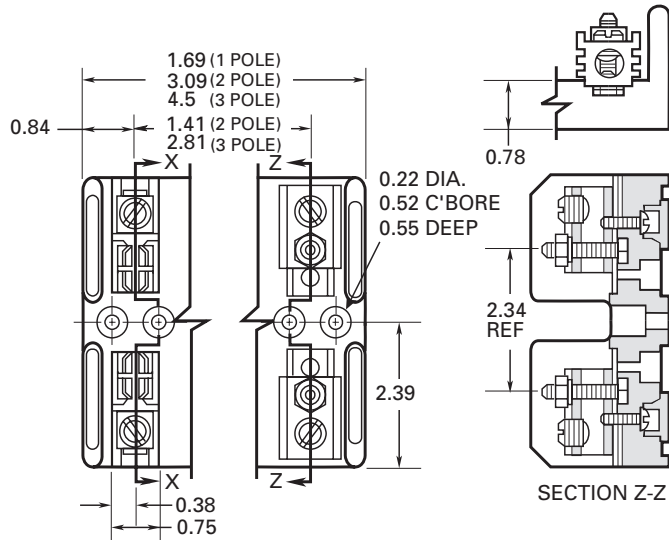
Figure 3. 61 to 100 A
