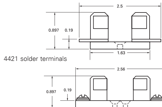
4515 with screw terminals
