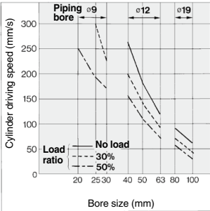
AS4000-02/03/04
