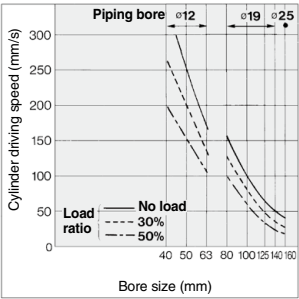
AS600-10
