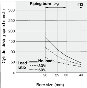
AS4000-02/03/04
