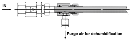
Semi-standard With fitting for purge air discharge (Semi-standard: P)
