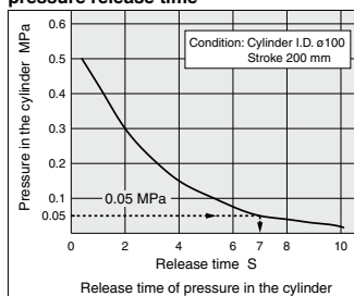
With One-touch fitting without a push button guard
