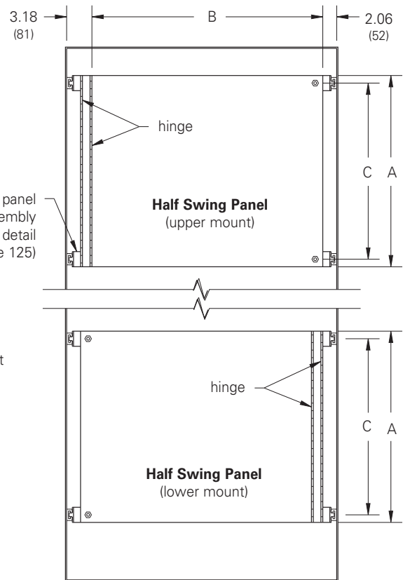
Half Swing Panel Mounting
