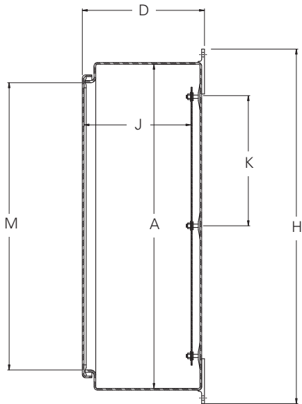
Section X-X
