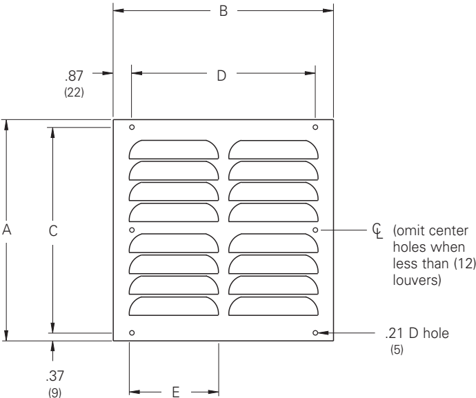
LPK84 to LPK812 Typical
