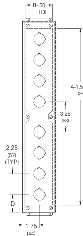
PV Series Typical 8 & 10 Hole
