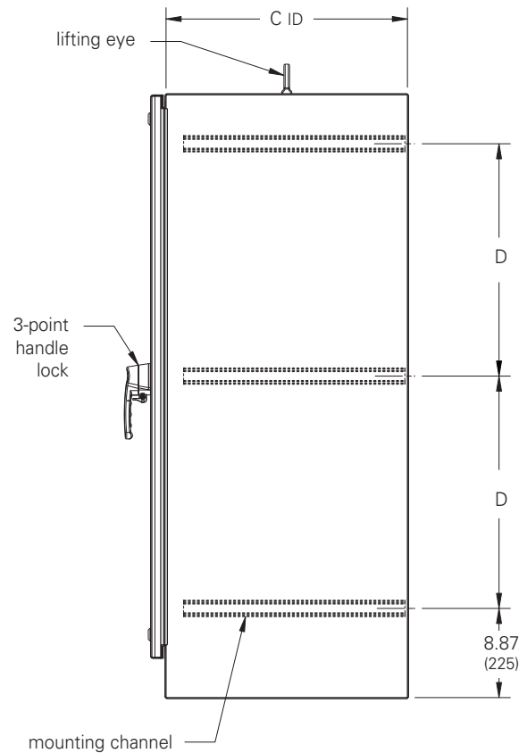
Side View
