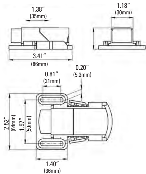
Dimensional Drawings
