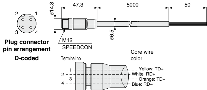
Connections
