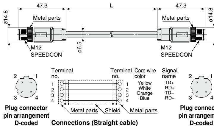
Connections (Straight cable)
