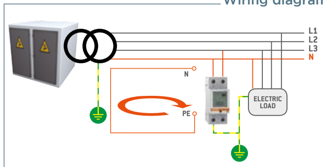
Wiring diagram
