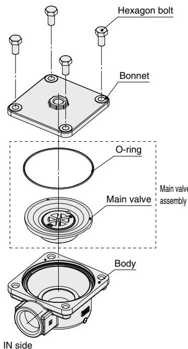
Fig. 2 O-ring position
