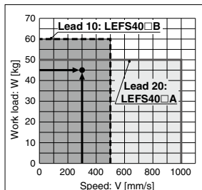
<Speed-Work load graph> (LEFS40)
