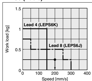
<Speed-Work load graph> (LEPS6/Step motor)
