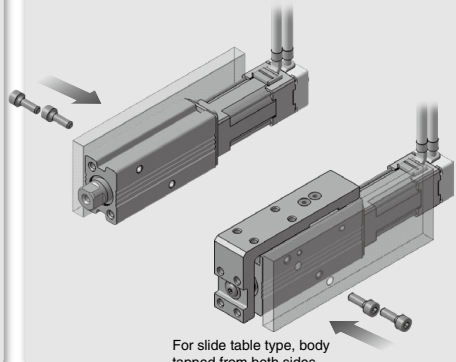
Side mounting (Body tapped)
