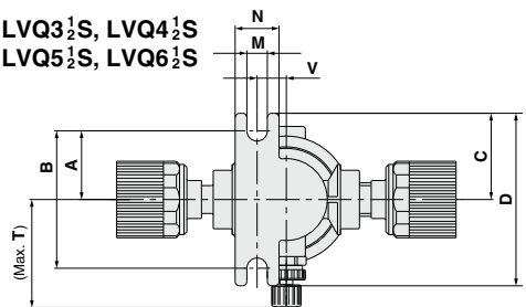
View Z
