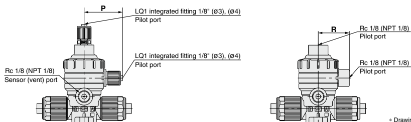
LVQ \square_2^1 -V \square Dimensions (N.O. Valve, Double Acting Valve)
