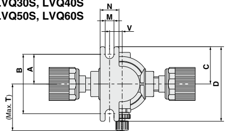
View Z
