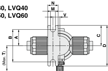
View Z
