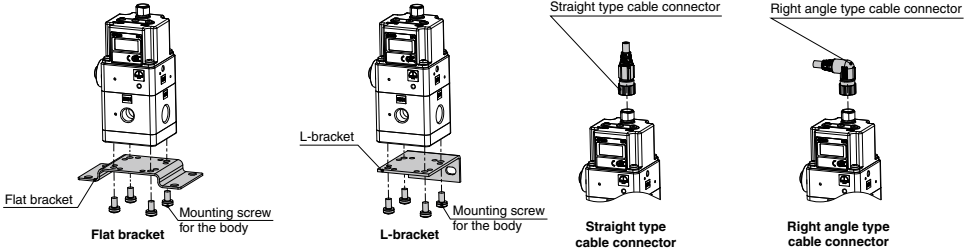
Flat bracket
