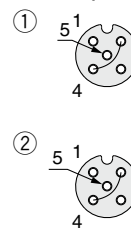
Socket connector pin assignment A-coded (Normal key)
