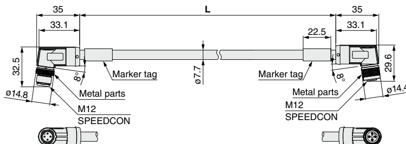
Socket connector pin arrangement A-coded (Normal key)
