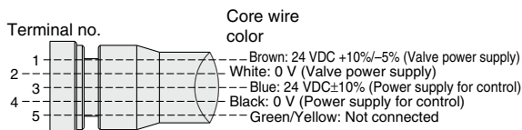
Connections (PROFIBUS DP/EtherCAT/PROFINET)
