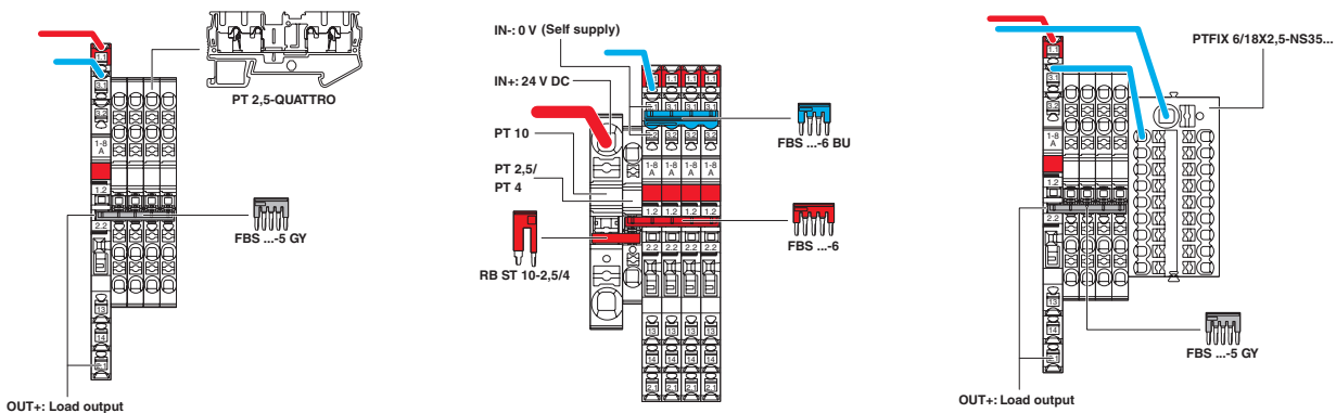
Bridging to adjacent CLIPLINE Complete terminal blocks
