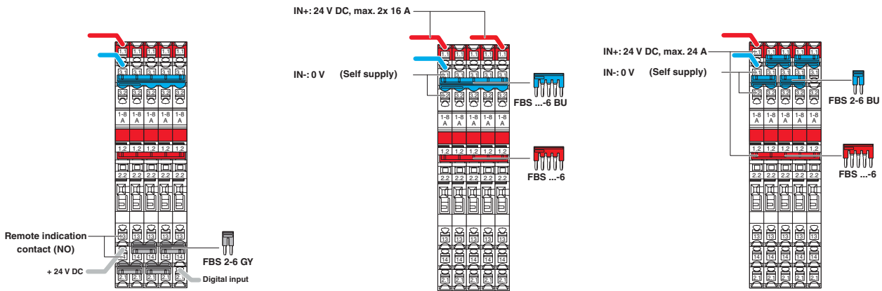
Bridging to adjacent PTCB
