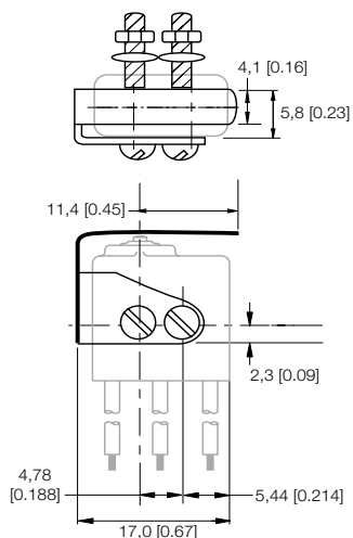
Figure 11. JM-1 Dimensions
