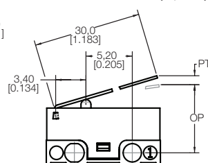
TYPE J LONG STRAIGHT LEVER (30,0 mm)
