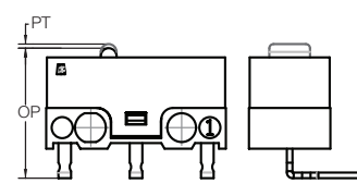
OP FROM TERMINAL (FOR TYPE 50 & 60 TERMINAL)
