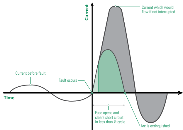
Figure 13 – Current-limiting Fuse
