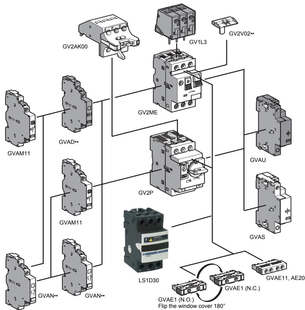
Figure 1: GV2 Accessories
