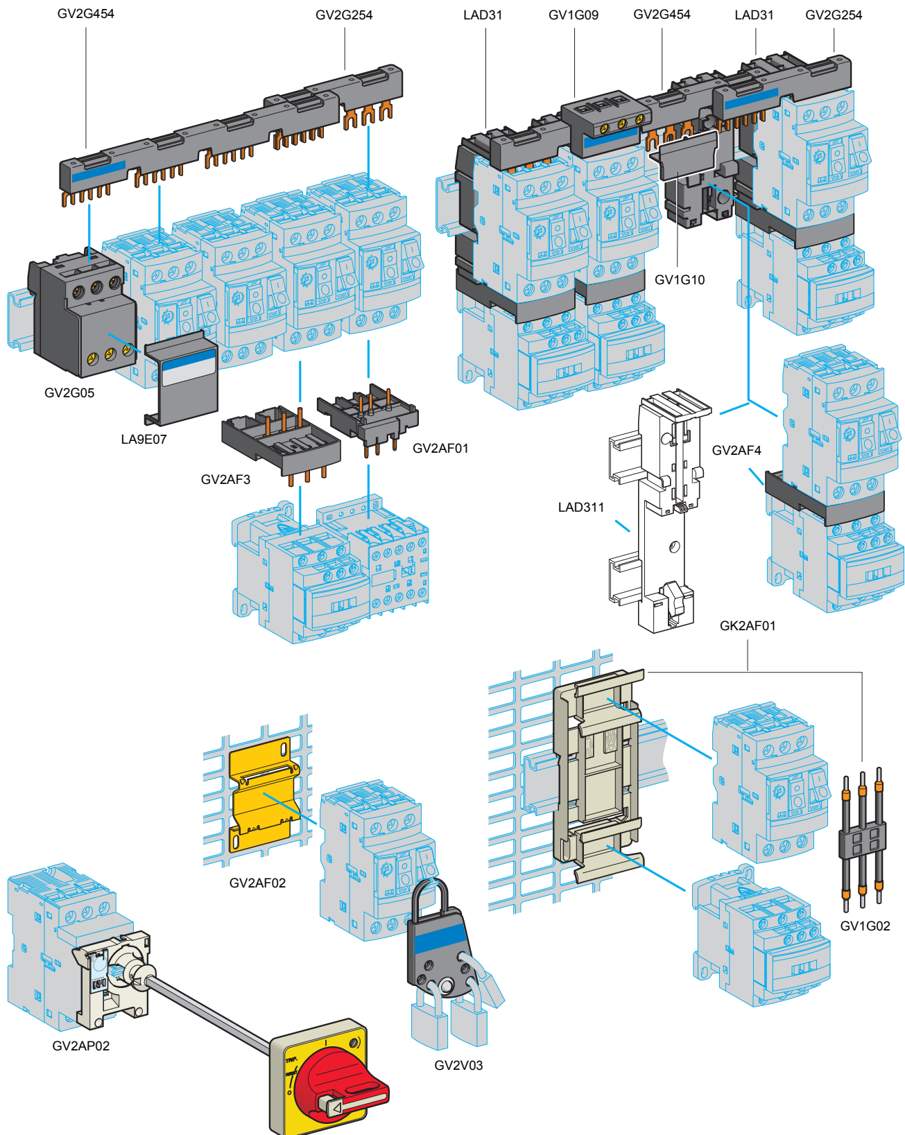
Figure 3: GV2 Accessories
