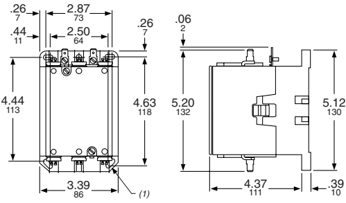
8910 DPA 70/90 (2 and 3-pole/75–90 A)
