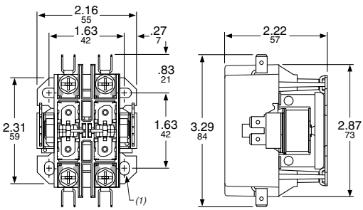
8910 DP 12/22/32/42 (2-pole)
