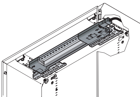
Mounting of LED system light
