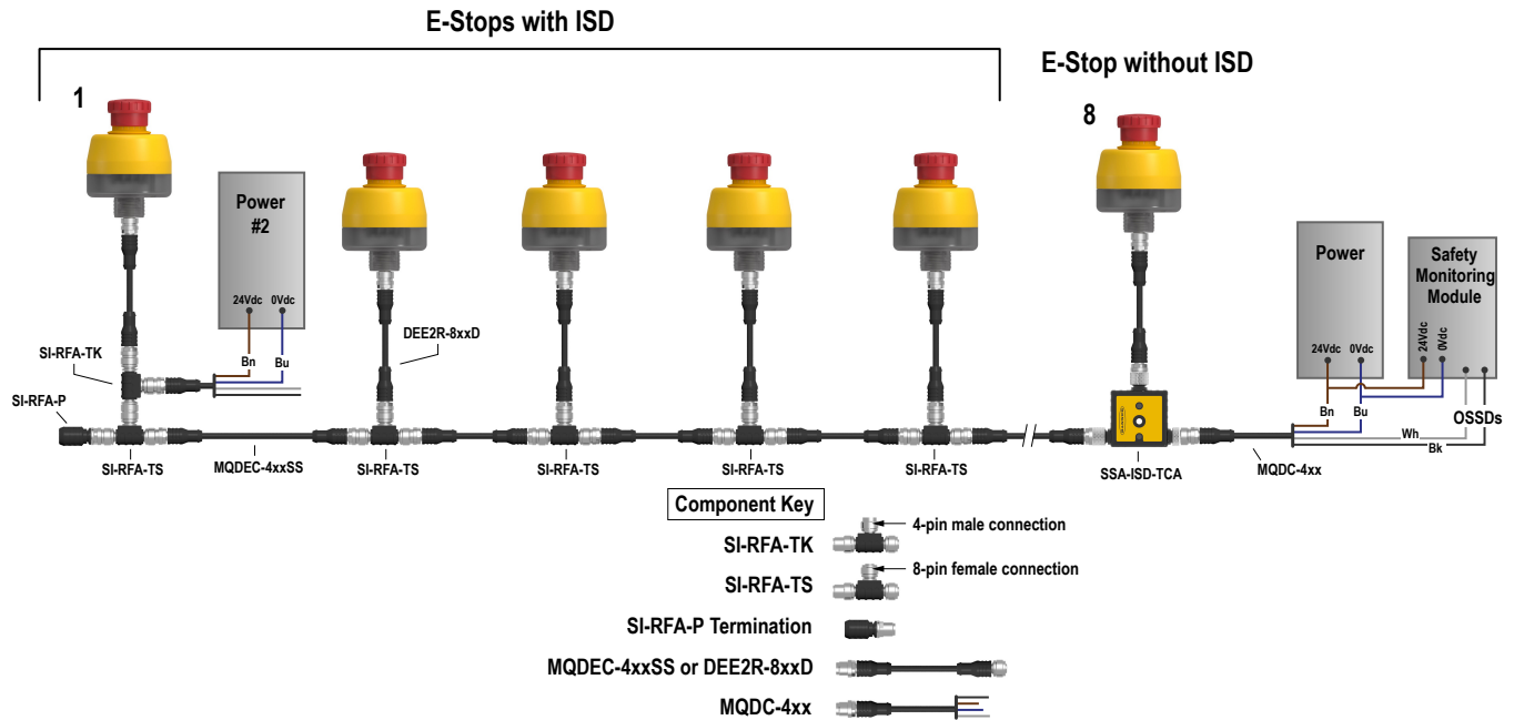
Figure 7. Option 2: Replace the terminator with a power supply. The OSSD1 and OSSD2 wires at power supply #2 must be connected to +24 V DC. If available, set the power supplies for parallel output.
