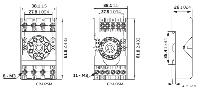
CR-U25M - CR-U35M - screw connection
