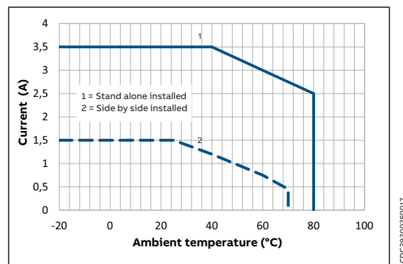
Triac output CR-P
