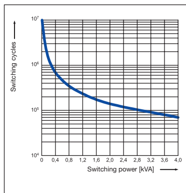
CR-P with 1 c/o contact
