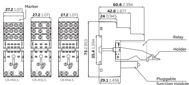
CR-M2LS - CR-M3LS - CR-M4LS - screw connection
