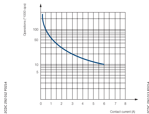
Endurance curve
