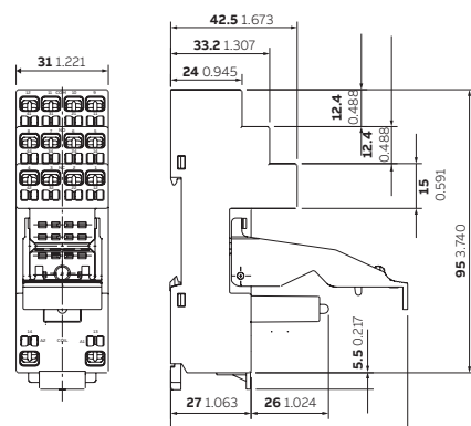
CR-M2LC, CR-M4LC - spring connection
