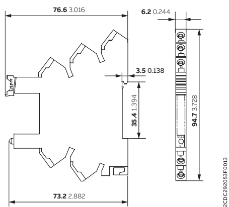
CR-S socket - spring connection
