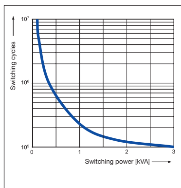
CR-M with 2 c/o contacts
