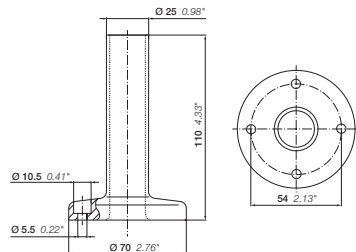
Base with integrated tube
