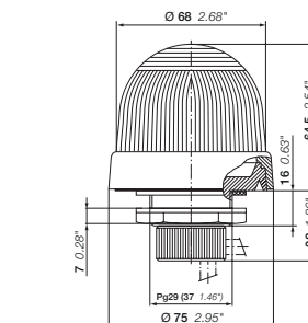
Signal beacons KSB
