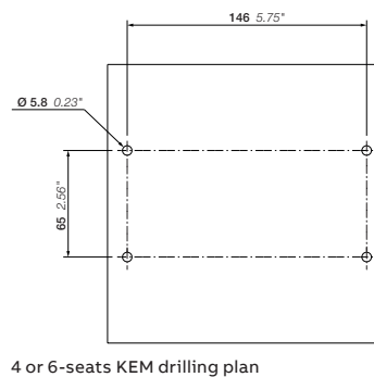
4 or 6-seats KEM drilling plan
