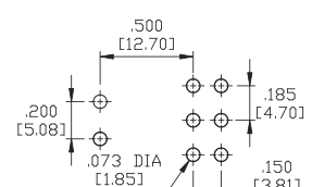
P.C.MOUNTING
