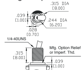
B6 High Torque
