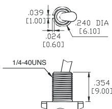
B1 Threaded B2 Non-Threaded
