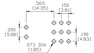
P.C.MOUNTING
