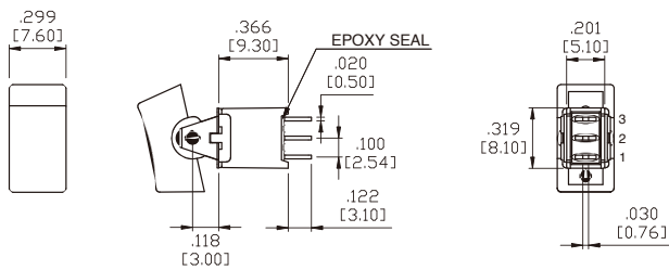
Single Pole
