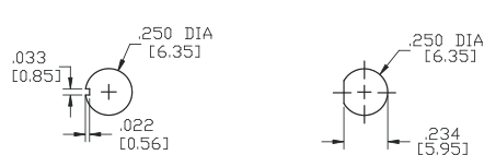
1/4 INCH BUSHING
