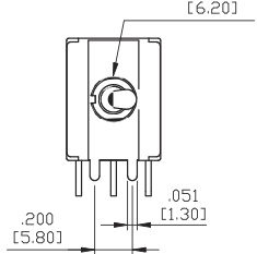
M6 Three Pole
