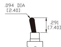
P4 Plastic Toggle
