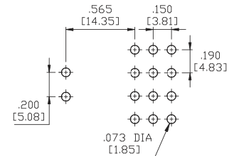
P.C.MOUNTING
