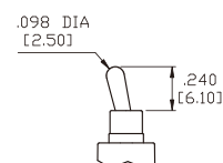
P3 Plastic Toggle
