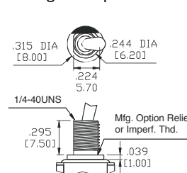
B5 High Torque
