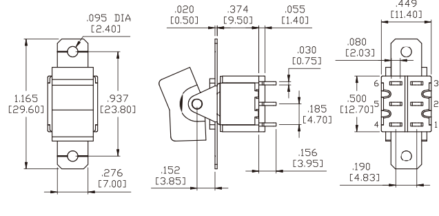
Double Pole
