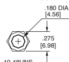
STANDARD .200
