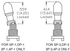
Locking Lever TA
