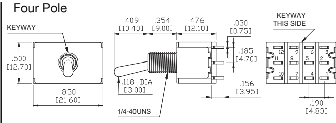
Four Pole
