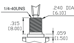
BA Threaded for T6
