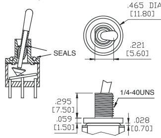
B9 Splash-Proof
