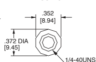
DRESS NUT
