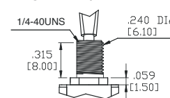
BB High Torque for T6
