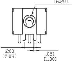
M7 Three Pole
