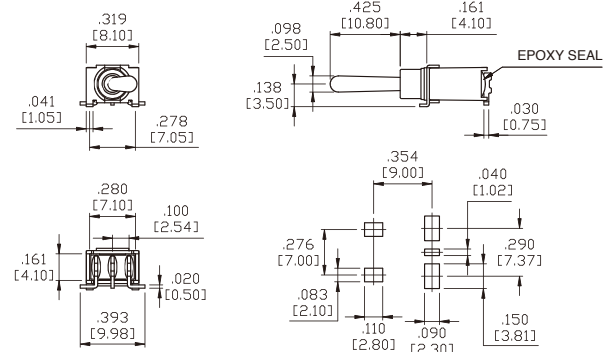
M7 Single Pole
