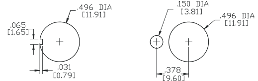
15/32 INCH BUSHING
