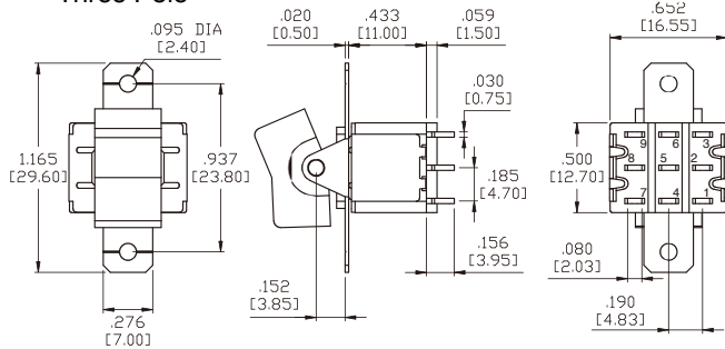
Three Pole
