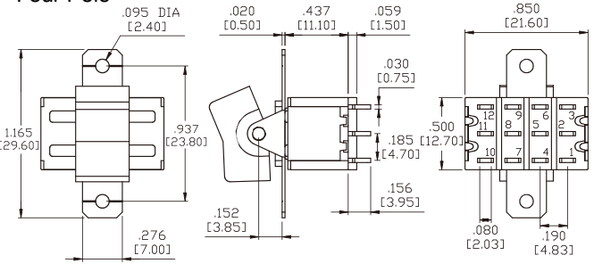
Four Pole
