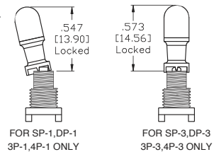
Locking Lever TL
