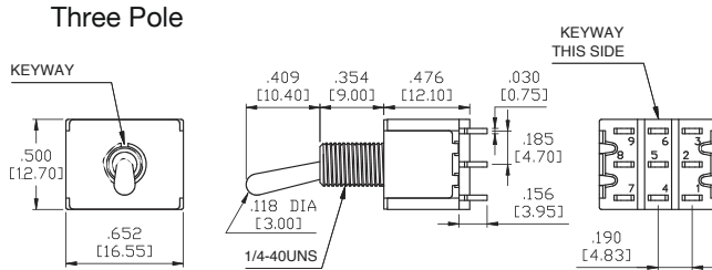
Three Pole
