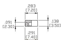
Plunger Caps
