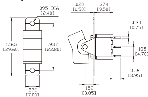
Single Pole
