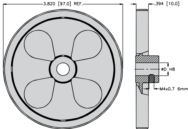
Measuring Wheel No. A9
