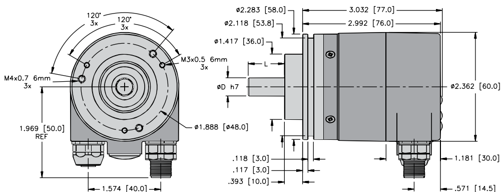
RM-29 Flange C Connection R2M12
