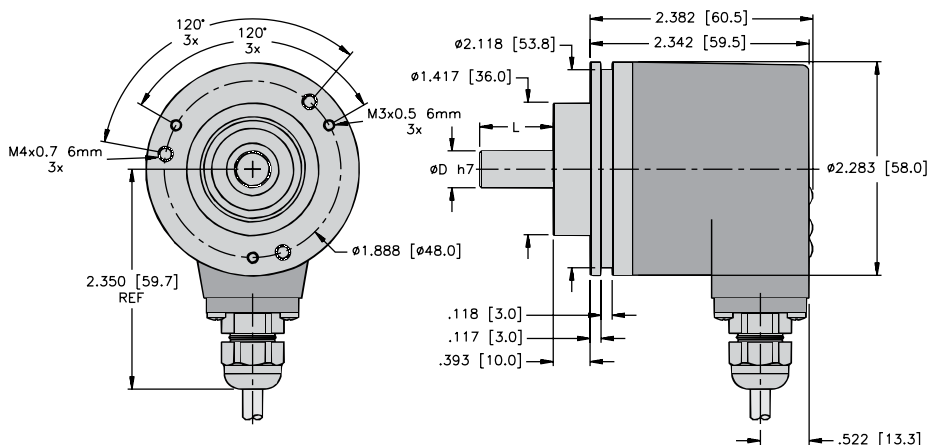
RM-29 Flange C Connection BC
