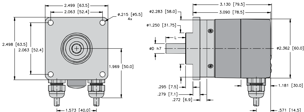
RM-29 Flange R Connection RC
