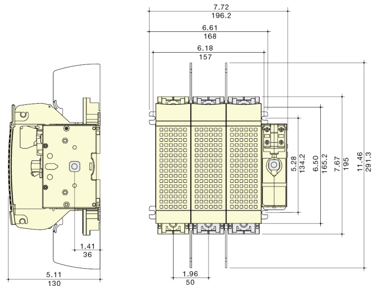
GS2QU3N, 400 A Fusible Disconnect Switches, Class J Fuses
