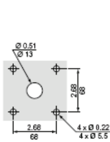
Four-hole mounting
