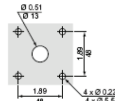
Four-hole mounting
