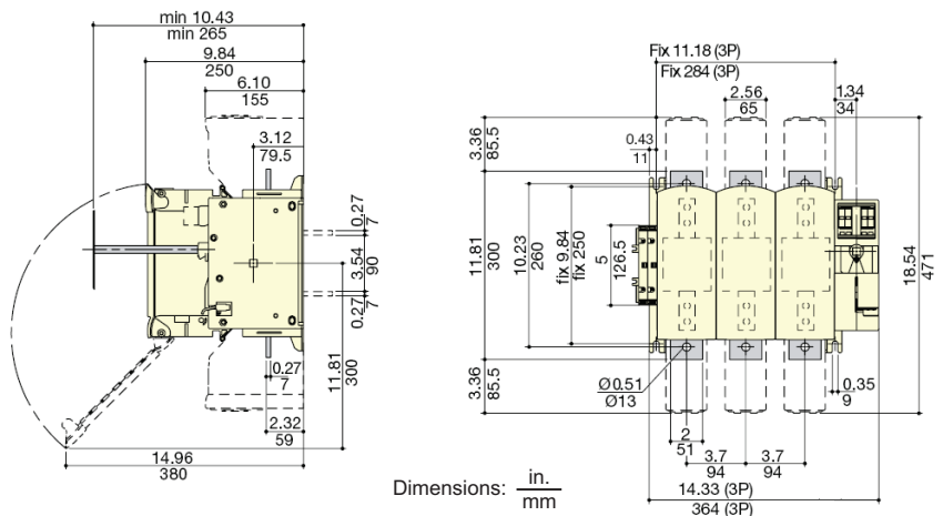
GS2SU3, 600 A Fusible Disconnect Switches, Class J Fuses GS2TU3, 800 A Fusible Disconnect Switches, Class J Fuses
