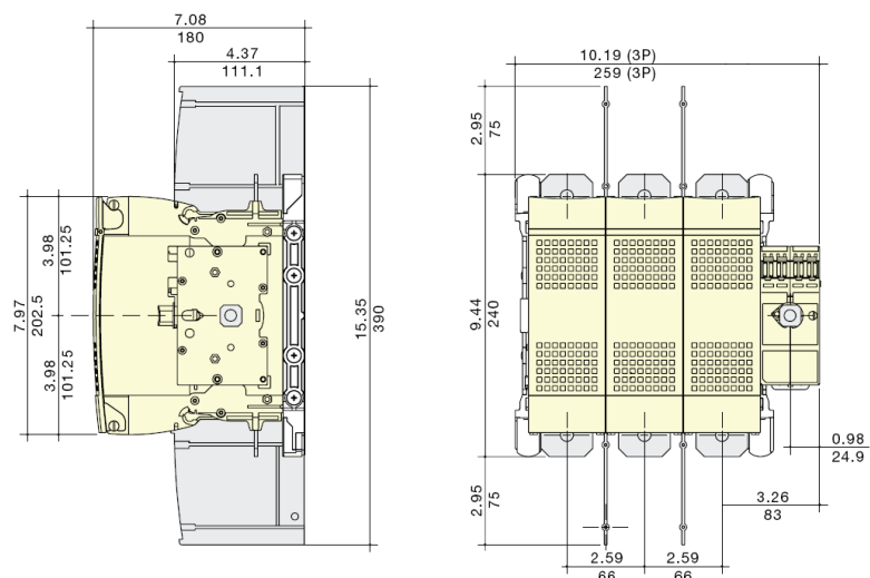
GS2SU3, 600 A Fusible Disconnect Switches, Class J Fuses GS2TU3, 800 A Fusible Disconnect Switches, Class J Fuses
