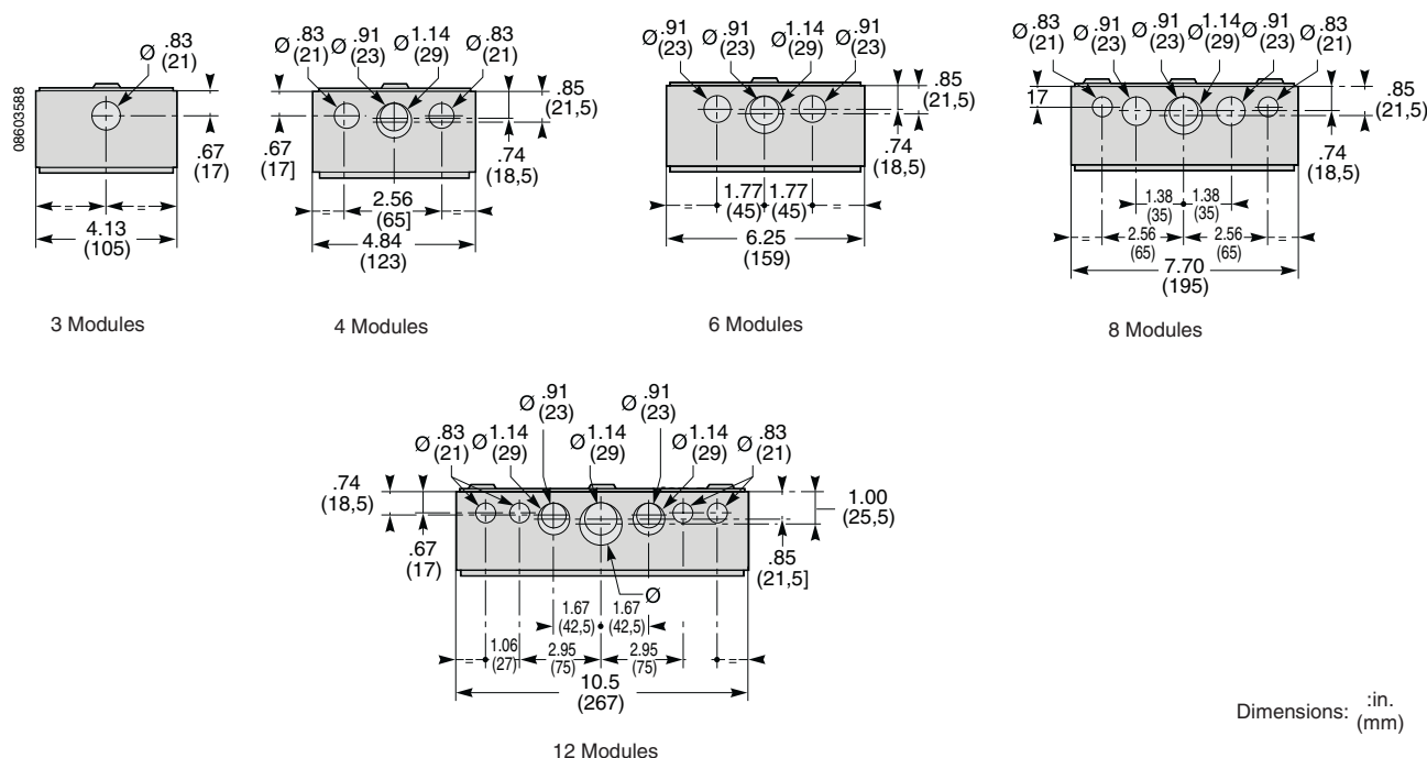
Figure 78: Top View for Kaedra Weatherproof Type Mini Enclosures
