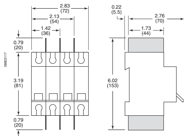
Figure 57: Interphase Barriers for C60 Devices
