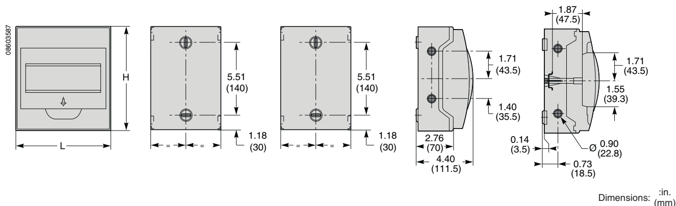
Figure 77: Kaedra Weatherproof Mini-Enclosures
