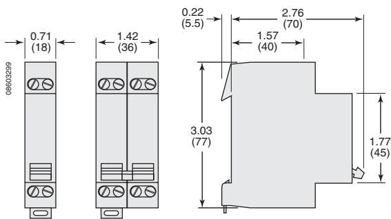
Figure 71: I Switch (20–32 A)
