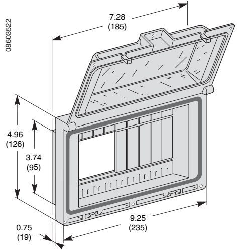
Figure 66: Multi-Pole Front Mounting Kit for C60 Devices
