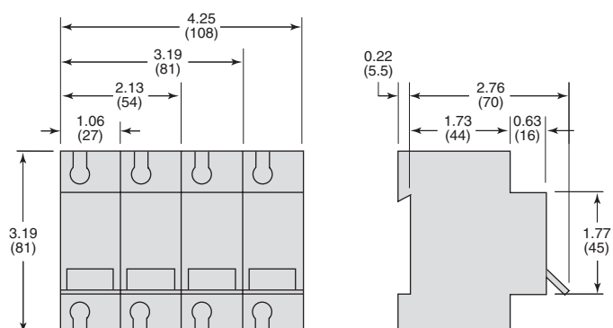
Figure 49: C120 IEC Circuit Breaker
