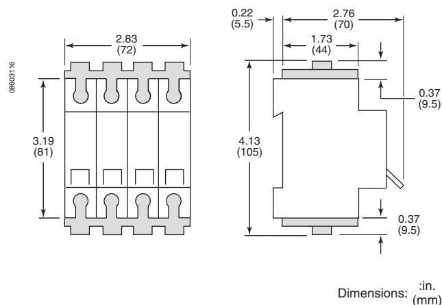
Figure 58: Terminal Screw Shield for UL 489A, UL 1077 and IEC C60 Devices
