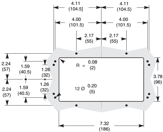
Figure 68: M9PF4 Pole Filler
