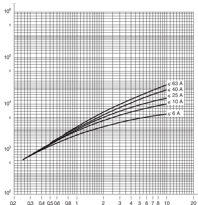
Figure 95: UL 489/CSA C22.2 No.5 Listed and UL 1077 Recognized C60 2P, 3P, and 4P (240 Vac) Max I^2t Peak Current
