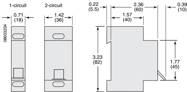
Figure 70: CM Switches
