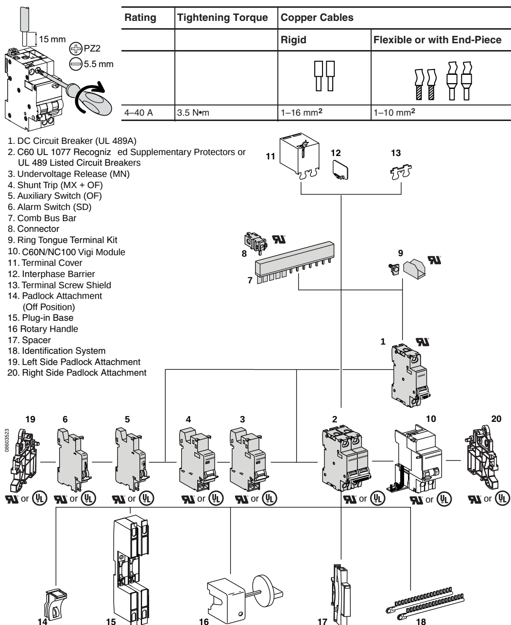
Figure 17: Overview of Multi 9 System Accessories
