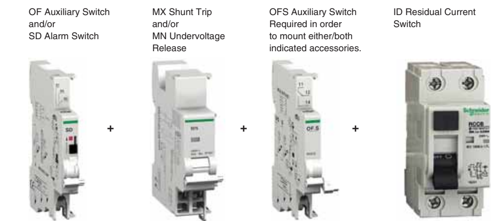
Figure 11: Possible Device Combinations
