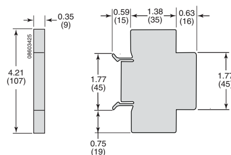
Figure 56: Spacer for C60 and C120 Devices
