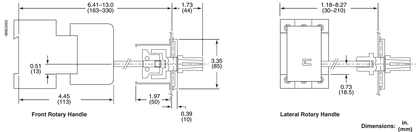
Figure 62: Rotary Handle for C60 Devices
