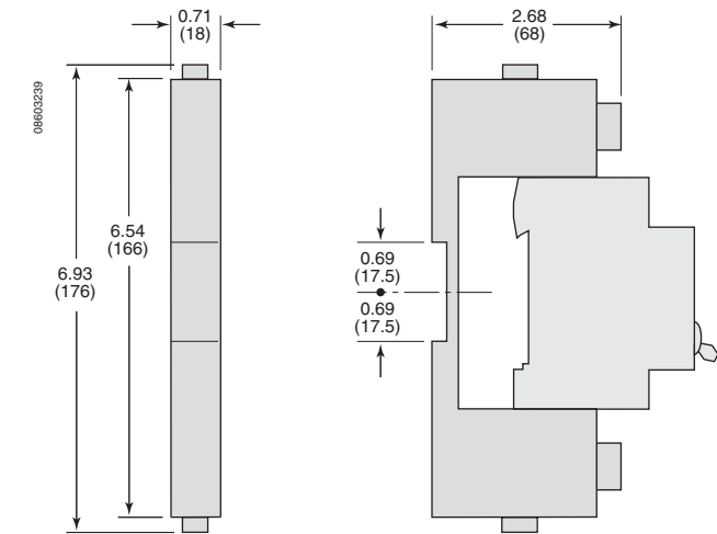
Figure 59: Plug-In Base for UL 489A, UL 1077 and IEC C60 Devices
