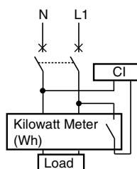
Figure 40: Schematics for IEC Rated CI Impulse Counter
