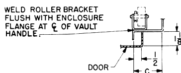
Welded Construction
