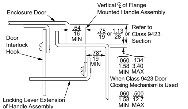
Flange Details
