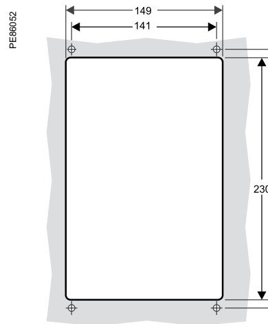
ION8650 switchboard mounting
