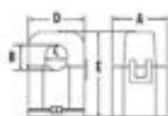
Split-Core CTs
