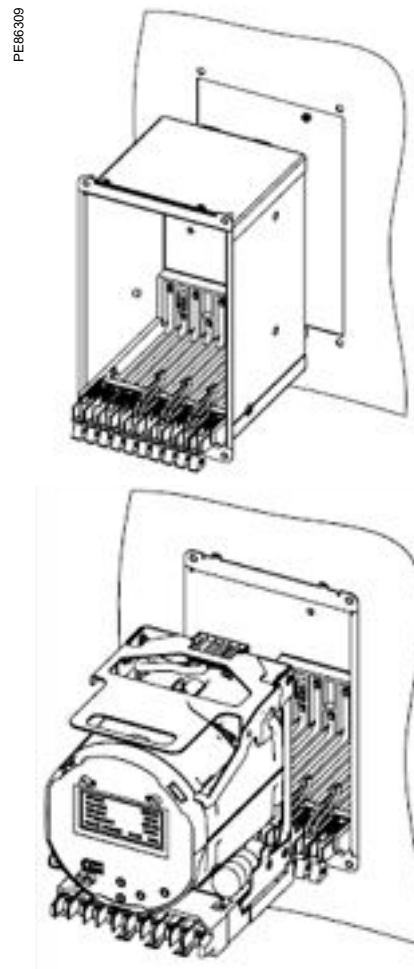
ION8650 switchboard mounting
