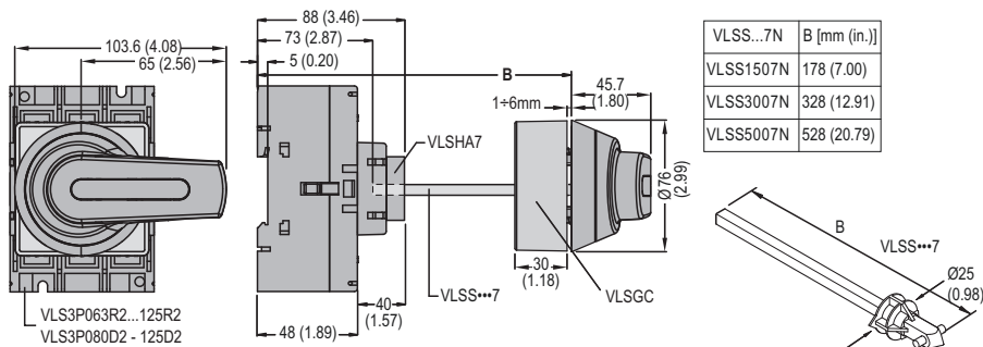
VLSS...7N used with VLHA7 and VLSH3S7NRD/BD
