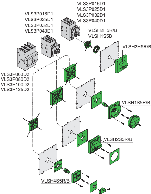
Figure 3: Door mounting version
