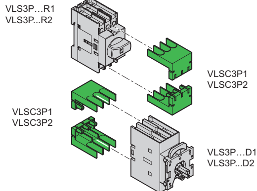
Figure 4: Terminal covers
