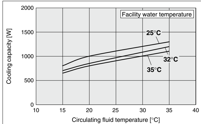
HRR012-A- 10 20 , HRR012-W- 10 20
