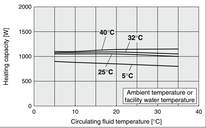
HRR050-A-20, HRR050-W-20 [50 Hz]
