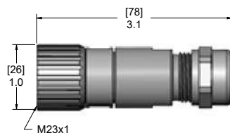
Straight Female Plug
