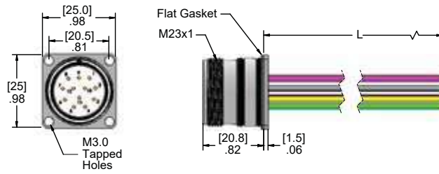
Female Receptacle
