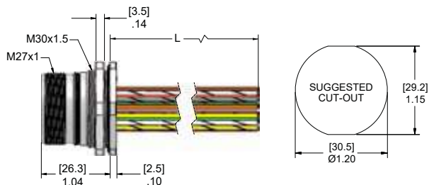
Back Mount
