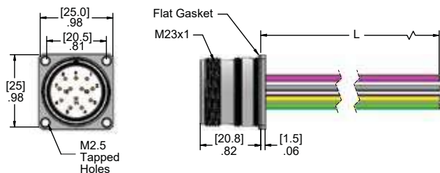
Male Receptacle
