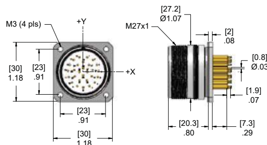
PCB Rear Mount
