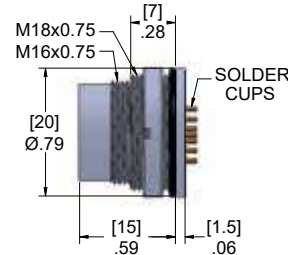
Male Receptacle
