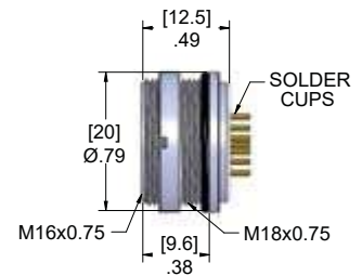
Female Receptacle
