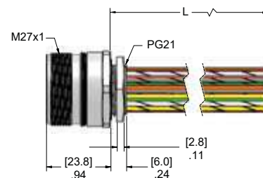
PG21 Threads
