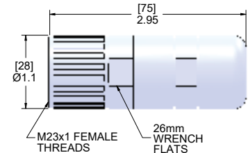
Female Plug with Female Threads
