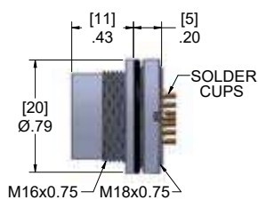
Male Receptacle
