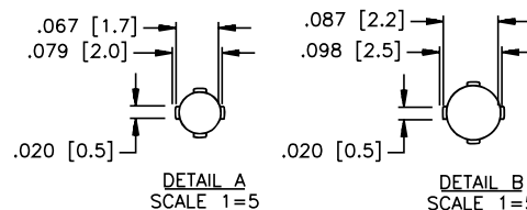
FSFDH - Detail
