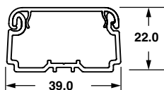
LDPH10 Internal Area = .62 Sq. In.
