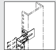
FZBA1.5X4 – Adjustable "Z" Bracket (page J.48)
