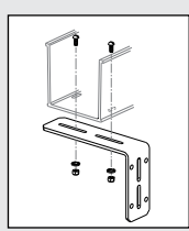
FLB – "L" Wall Mount Bracket (page J.48)
