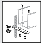
FTRBE12 – Existing Threaded Rod Bracket (page J.48)
