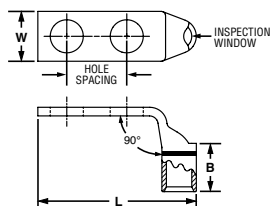
Figure 3: 90° Bent
