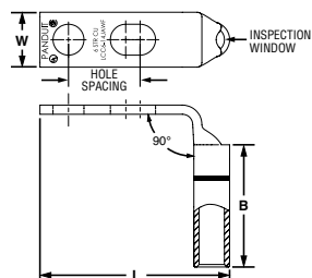
Figure 6: Slotted, 90° Bent
