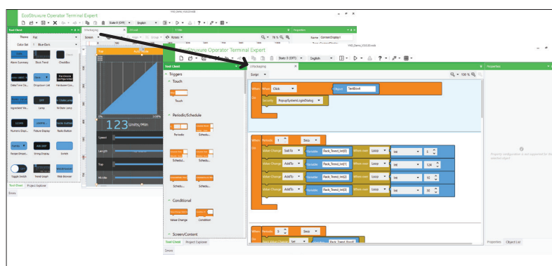
Block scripting
