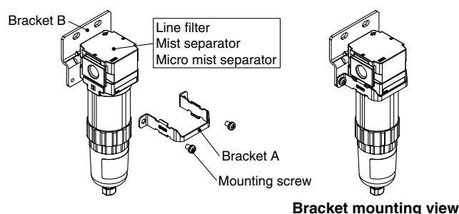
Bracket mounting view
