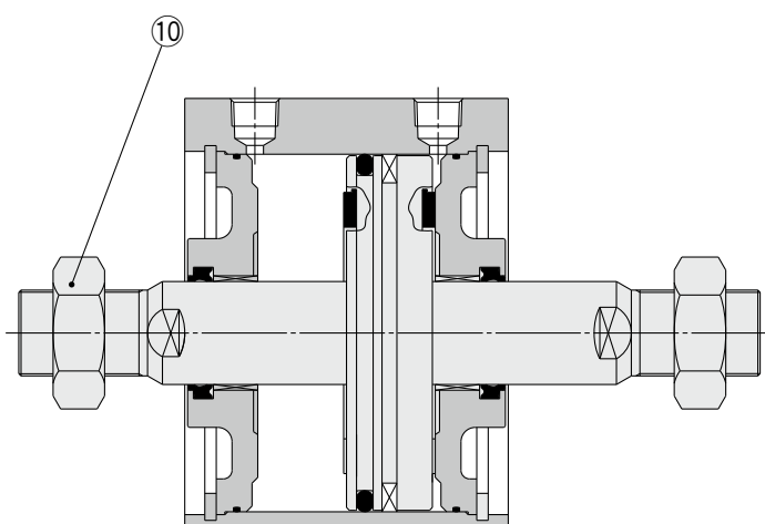
Rod end male thread
