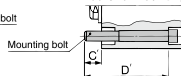
Rod end mounting
