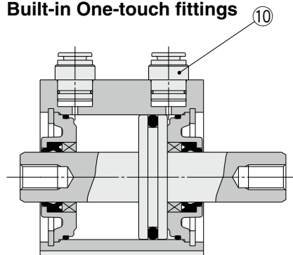
Built-in One-touch fittings
