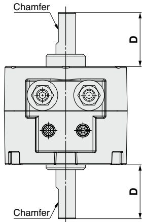
Double shaft/CRBY□
