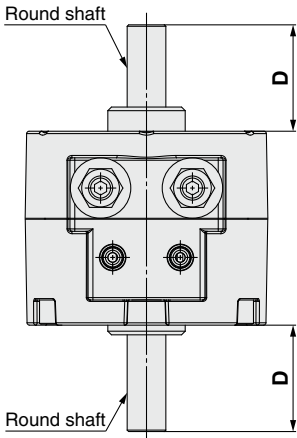
Double shaft/CRBK□
