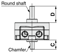
Double shaft/CRBJ□
