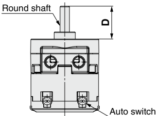
Single shaft/CDRBT□
