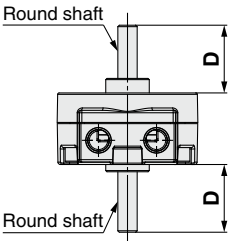
Double shaft/CRBK□
