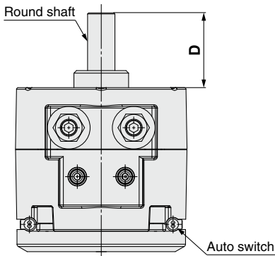
Single shaft/CDRBT□
