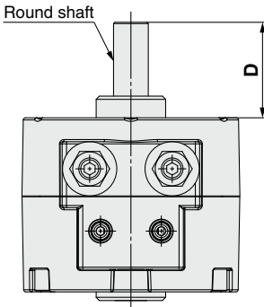
Single shaft/CRBT□
