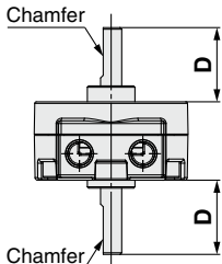
Double shaft/CRBY□
