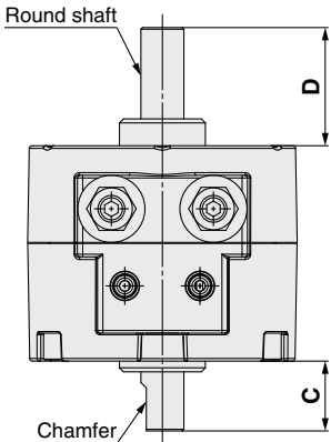
Double shaft/CRBJ□
