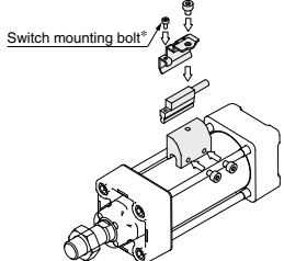
<Mounting example for ø32, D-P3DWA>
