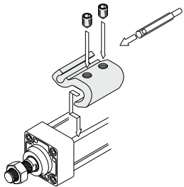
<Mounting example for ø32, D-P3DWA>
