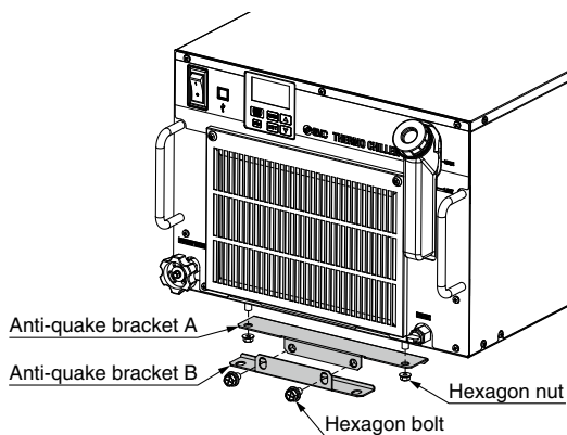
Mounting view
