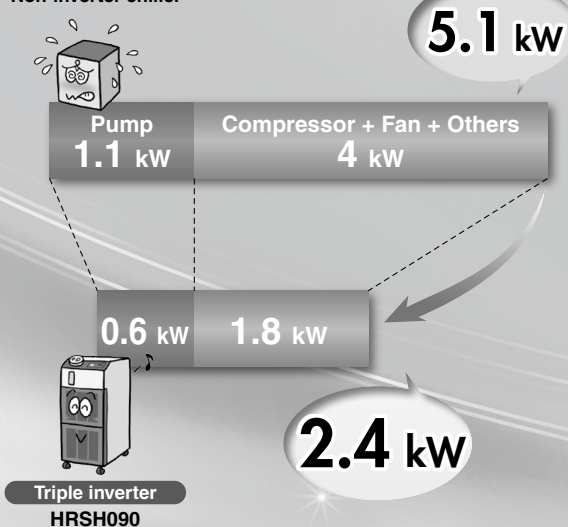
Non-inverter chiller
