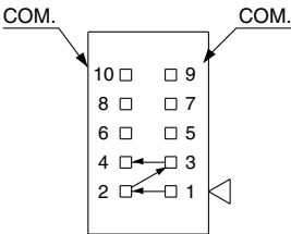
(PH, PHC: 10 pins)
