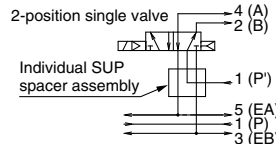
Circuit diagram (Mounting example of a 2-position single valve)
