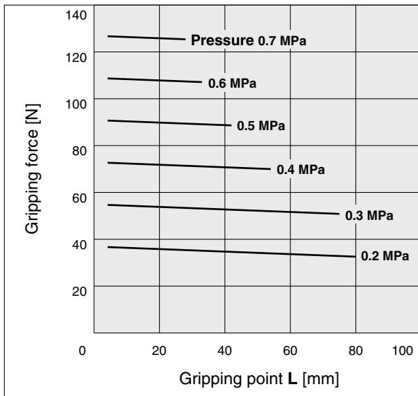
MHF2-16FD□
