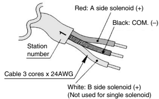
Lead wire assembly with connector
