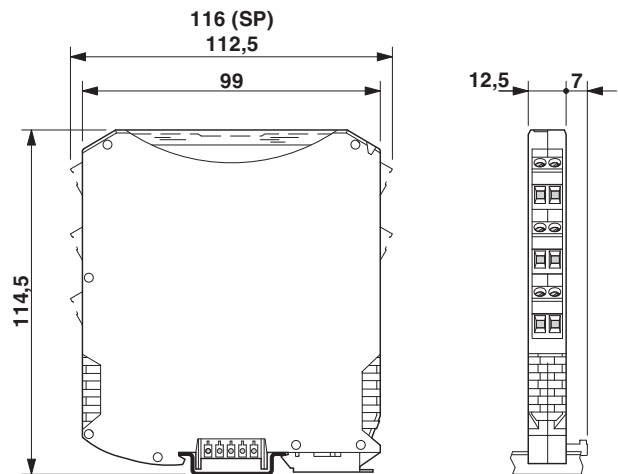
Figure 3 Dimensions
