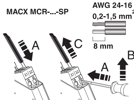
Figure 6 Push-in connection
